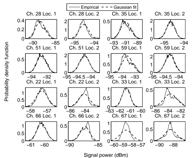
Fig. 6. Probability density function of signal power for analogical (28, 35, 51 and 59) and digital (22, 33, 66 and 67) TV channels.
