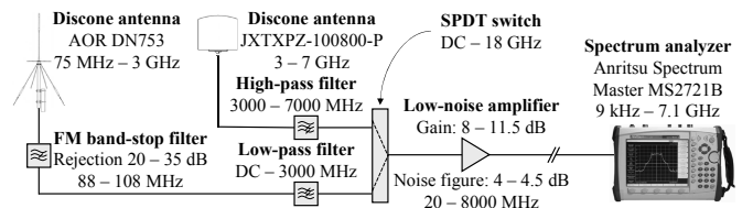
Fig. 1. Measurement setup employed in this study.
