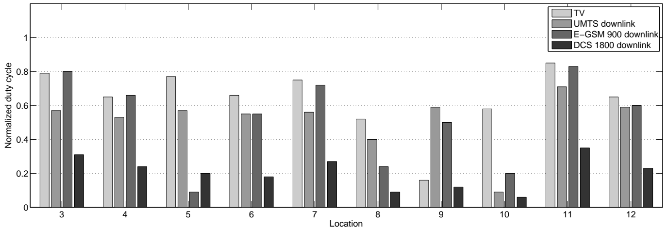
Fig. 4. Normalized average duty cycle statistics in locations 3 to 12 for specific bands: TV (470-862 MHz), UMTS downlink (2110-2170 MHz), E-GSM 900 downlink (925-960 MHz), and DCS 1800 downlink (1805-1880 MHz).
