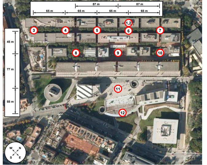
Fig. 2. Measurement locations in urban environment.
